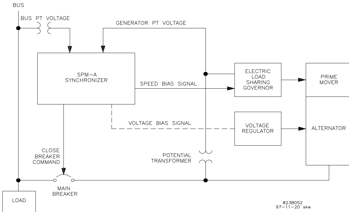
Synchronizer Functional Diagram
