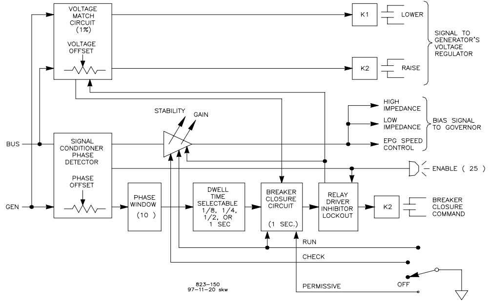
Synchronizer Block Diagram
