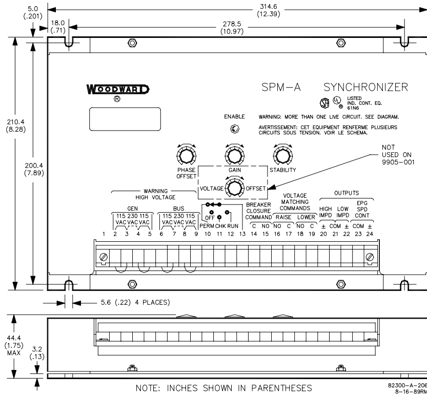
SPM-A Outline Drawing
