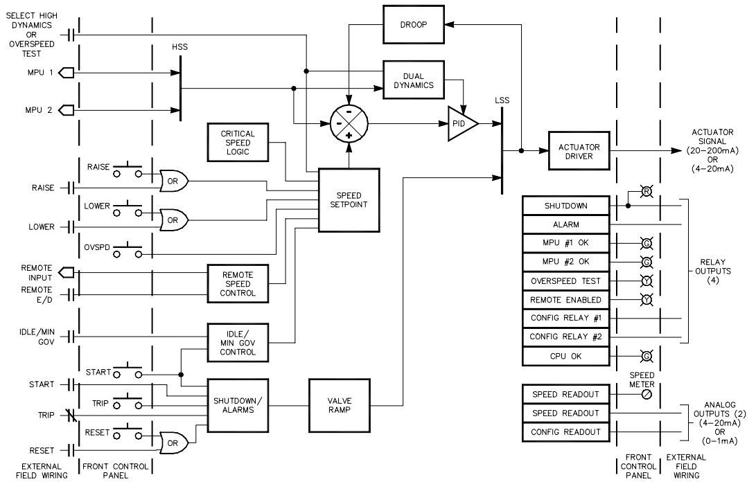
Block Diagram
